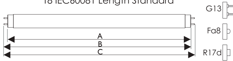
T8 IEC60081 Length Standard
