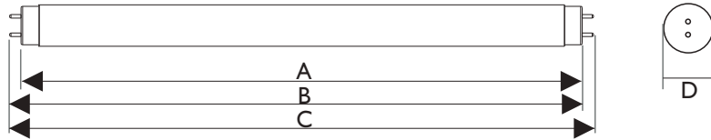
T5 IEC60081 Length Standard
